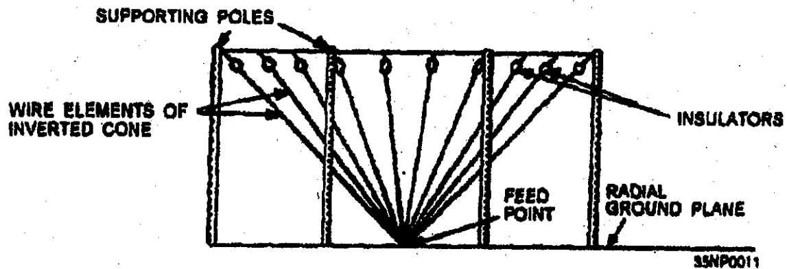
Inverted cone antenna.
